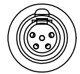
"P2" 5-PIN FEMALE CONNECTOR
